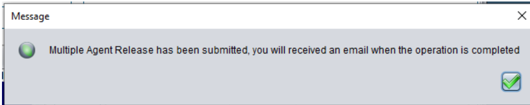
Figure 5: Message
