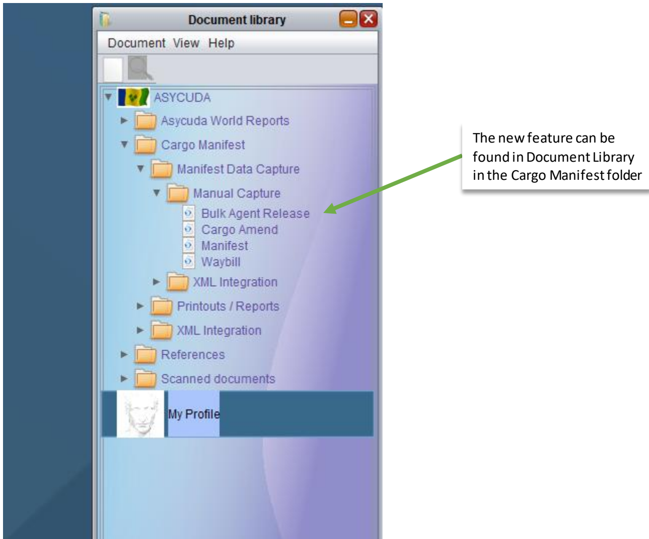
Figure 1: Document Library
